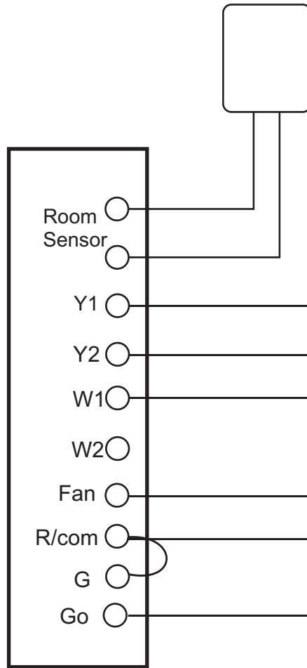
Smart Temp Model SMT-920 Viking Programmable Thermostat
